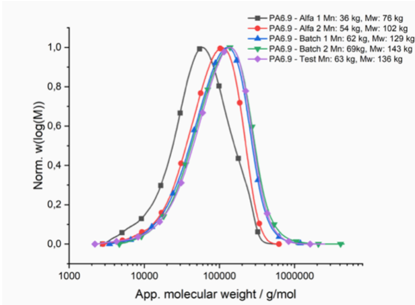
Figure 1 – Comparison of the molecular weight of commercially sourced polyamide 6.9 and algae-based polyamide 6.9 produced in the project.
