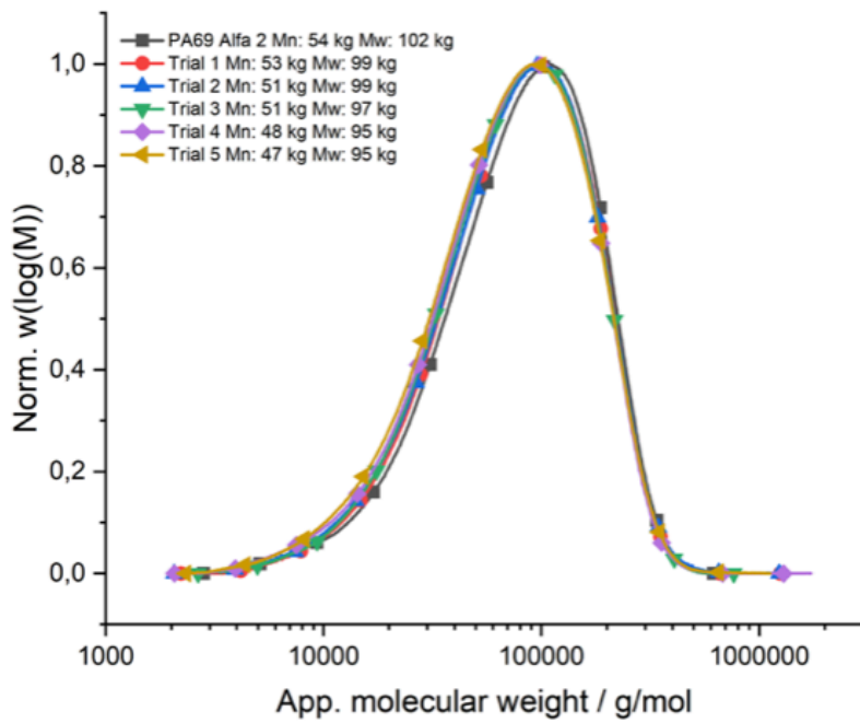
Figure 2 – Comparison of the molecular weights of commercial biobased polyamide 6.9 thermo-mechanically recycled 5 times.
